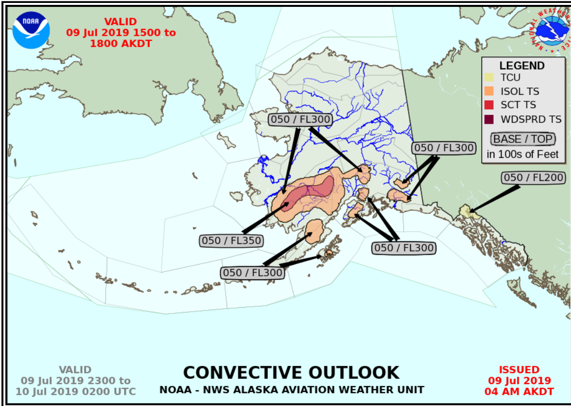
Figure 27-13. Alaska Convective Outlook
