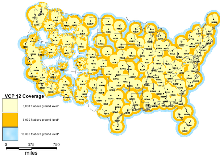
Figure 24-9. WSR-88D Weather Radar Coverage at 3,000 ft AGL, 6,000 ft AGL, and 10,000 ft AGL over the CONUS and Puerto Rico
