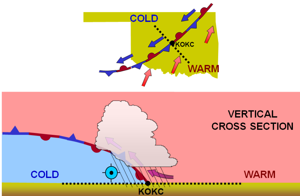
Figure 11-7. Stationary Front
