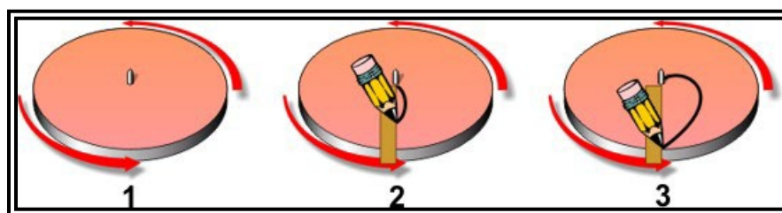
Figure 10-3. Illustration of Coriolis Force
