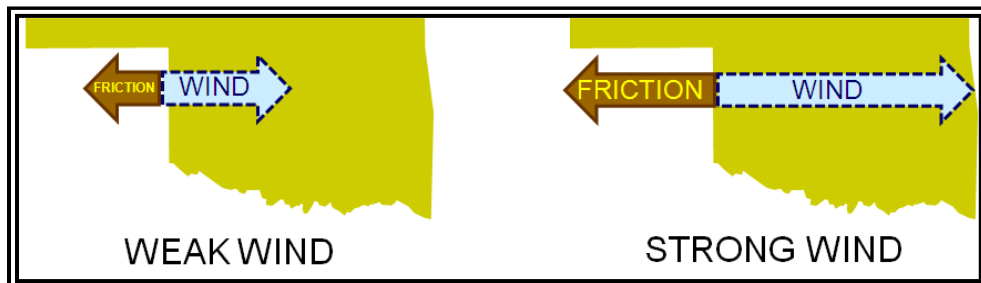
Figure 10-7. Friction Force Magnitude Variations with Wind Speed
