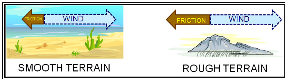
Figure 10-6. Friction Force Magnitude Variations with Terrain Roughness
