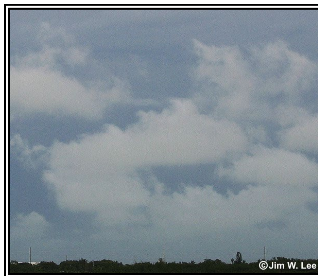
Figure A-12. Stratus Fractus (StFra) and/or Cumulus Fractus (CuFra) of Bad Weather
