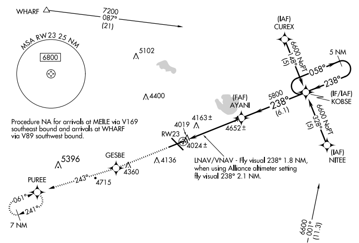
RNAV Approach
