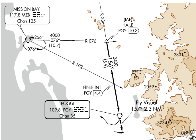
Traditional (NAVAID) Approach
